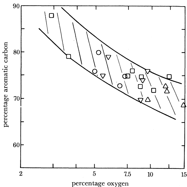
FIGURE 18. Correlation of aromaticity in a number of coals with oxygen content in the solvent-refined coal. \circ , West Kentucky; \square , Burning Star; \nabla , Monterey; \triangle , Wyodak.
